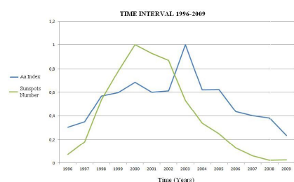
Figure 1: Normalized Aa index (blue) and sunspots number (green) as a function of time (years).
