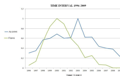
Figure 3: Normalized aa index (Blue) and the flares (Green) as a functions of time.
