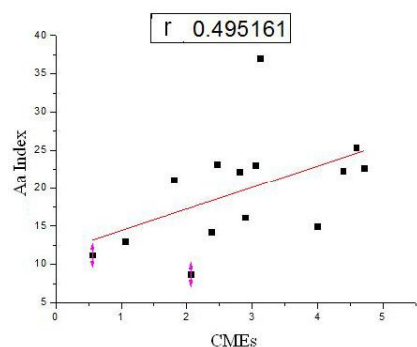
Figure 6: Dispersion Diagram between the aa index and the CME, for annual values.
