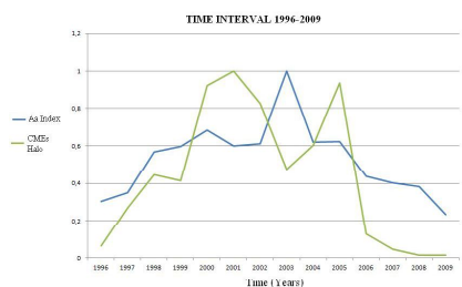
Figure 7: Normalized aa index (Blue) and Halo CME (Green) as a functions of time.
